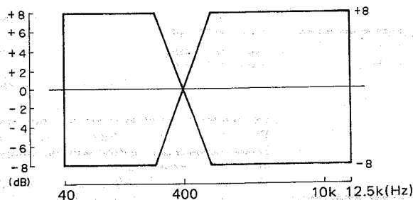
Fig. 5-10 Overall frequency response
