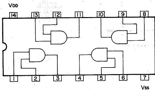
M4081BP
