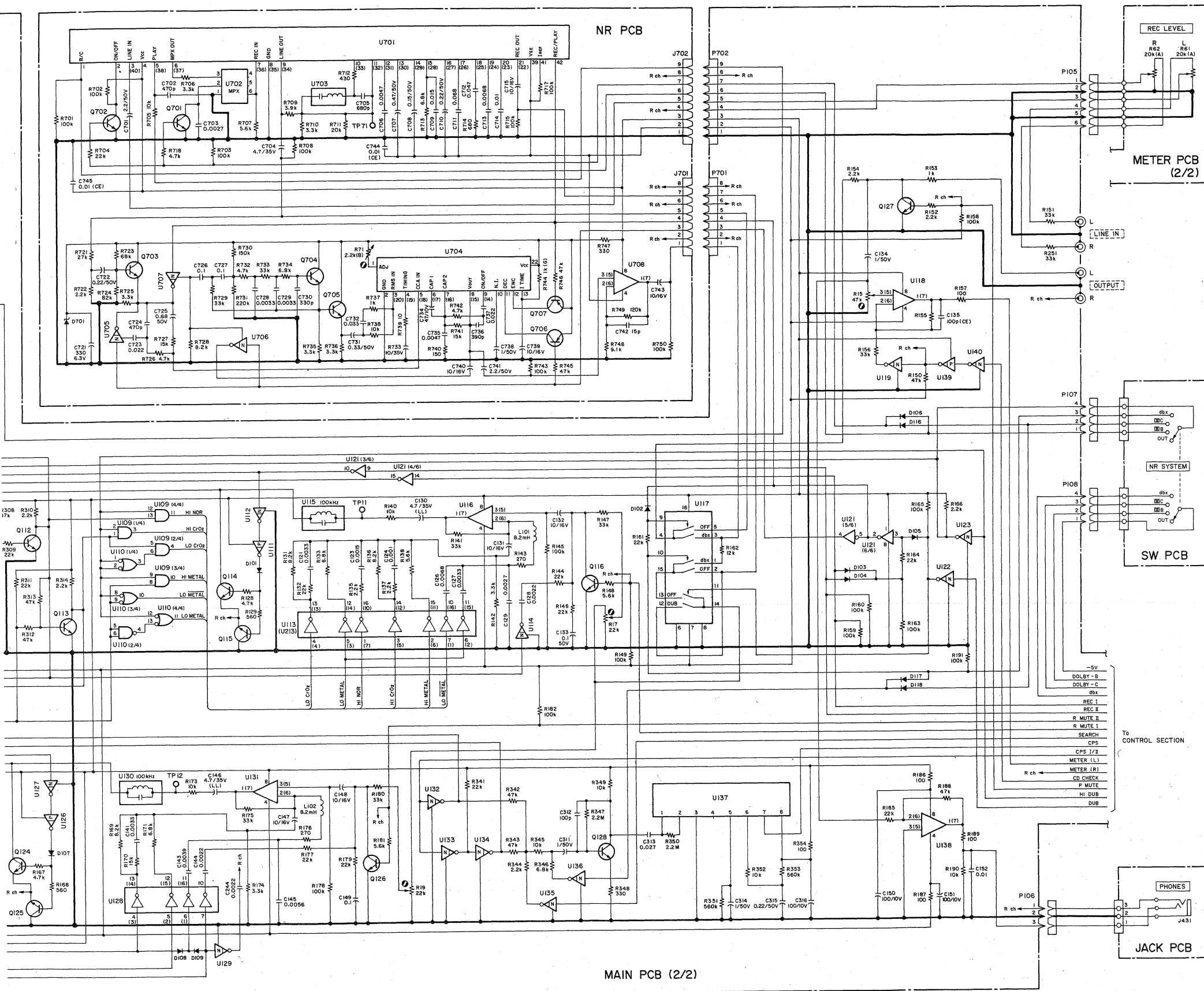
MAIN PCB (2/2)
