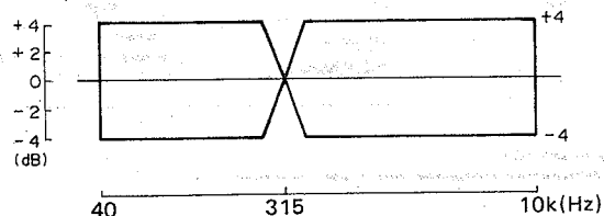
Fig. 5-8 Playback frequency response
