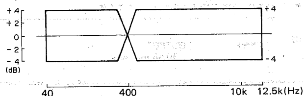
Fig. 5-9 Overall frequency response (Dolby NR: OUT)
