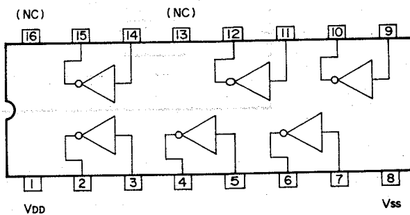
M4049UBP
