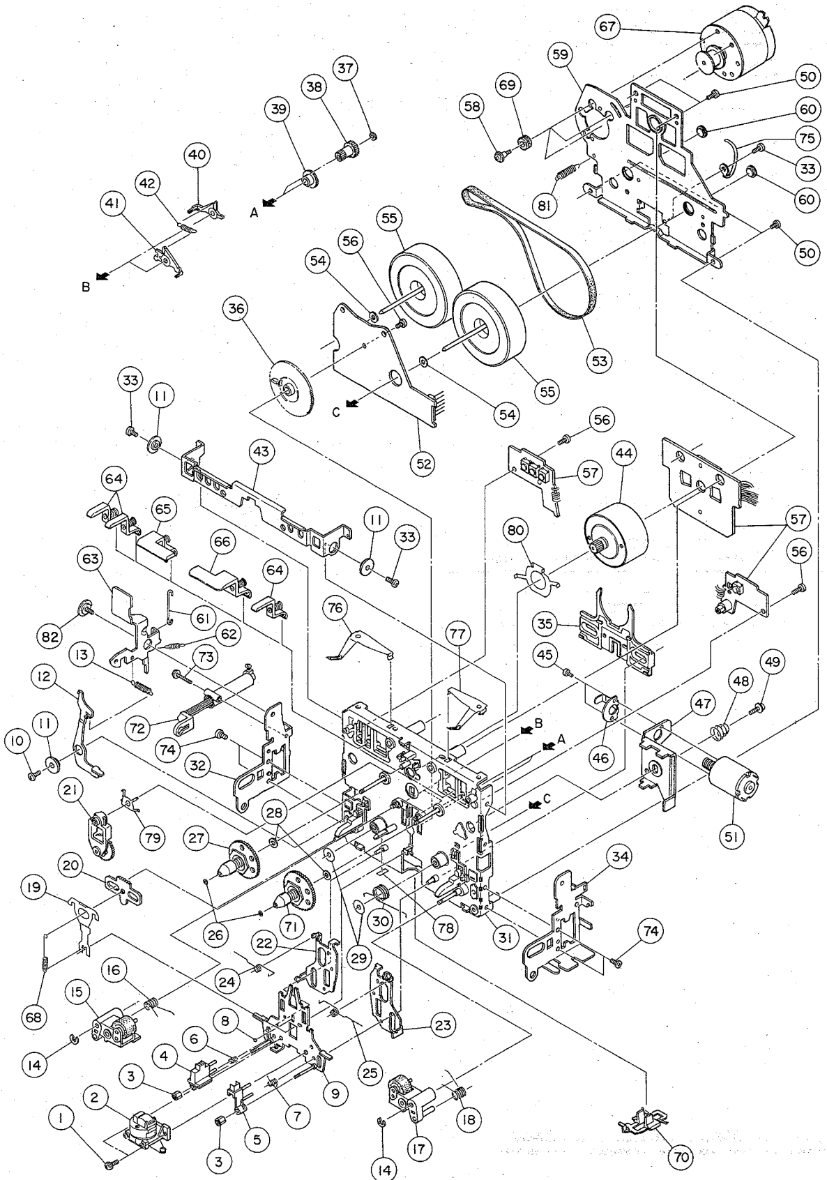
EXPLODED VIEW-2 (Deck I)
