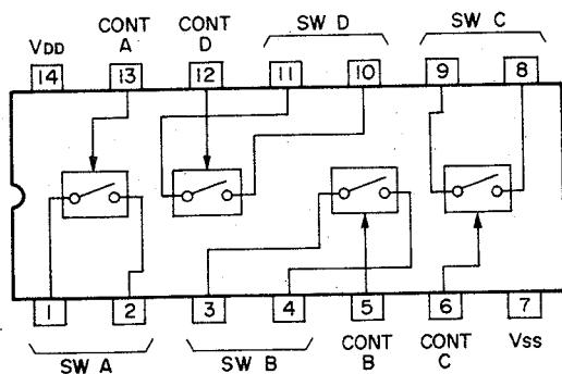
M4066BP
