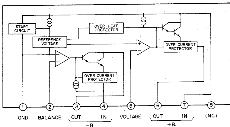
M5230L
