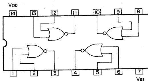
M4001BP
