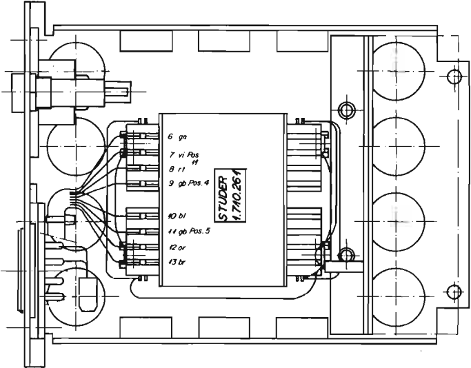
TRANSFORMER UNIT 1.710.260
