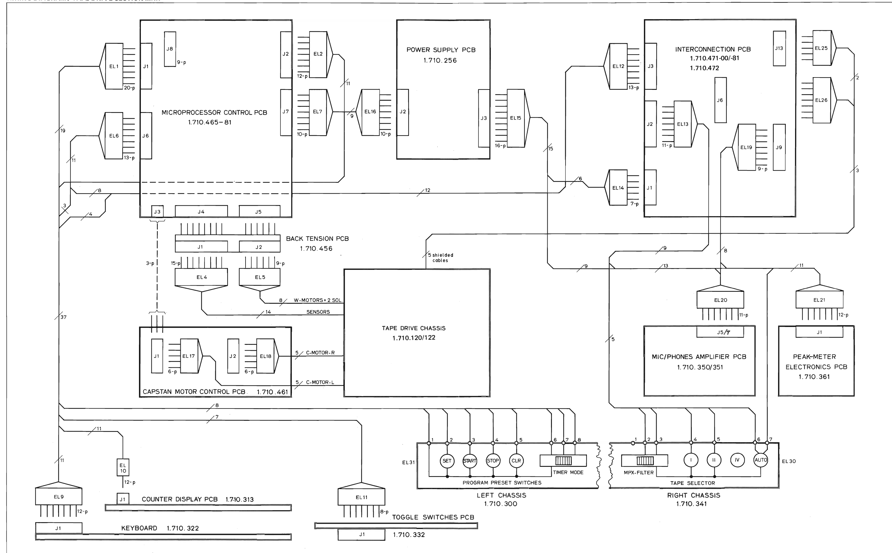
WIRING DIAGRAM / TAPE DRIVE SECTION MKII
