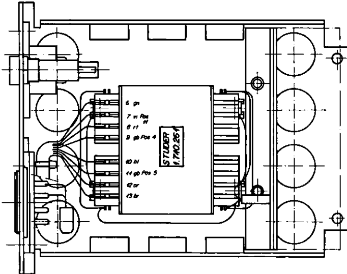
TRANSFORMER UNIT 1.710.260
